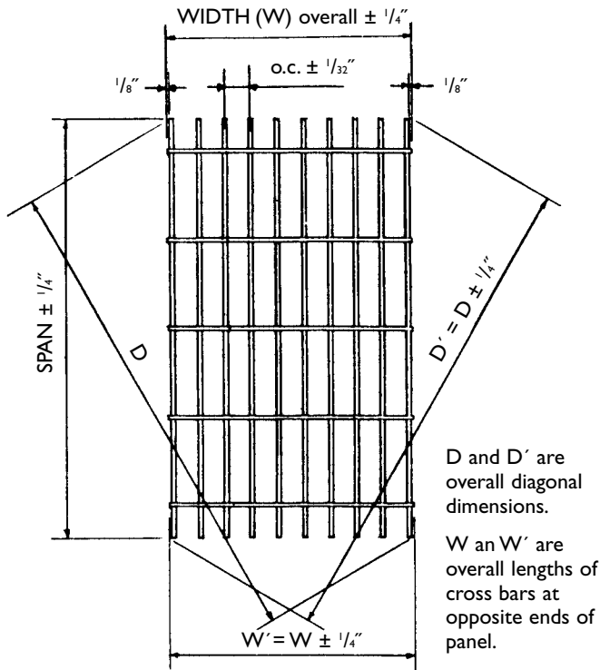
Overall Dimensions and Squareness
