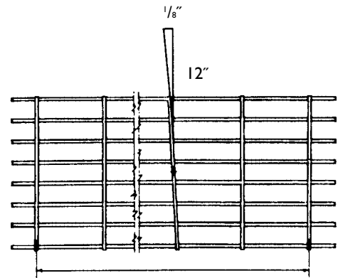
Cross Bar Alignment and Spacing
