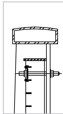
Section View
