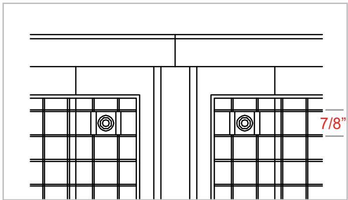
Detail - Panel Attachment View
