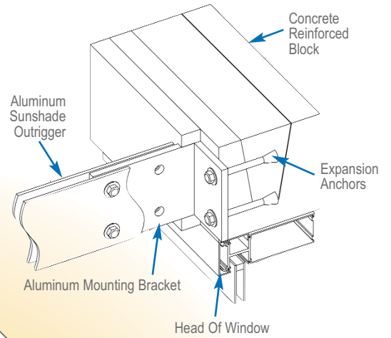
Concrete Lintel ▲
