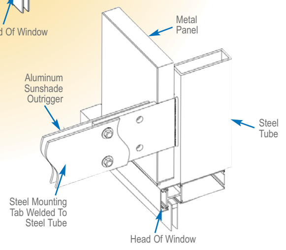
Welded - Curtain Wall ▲
