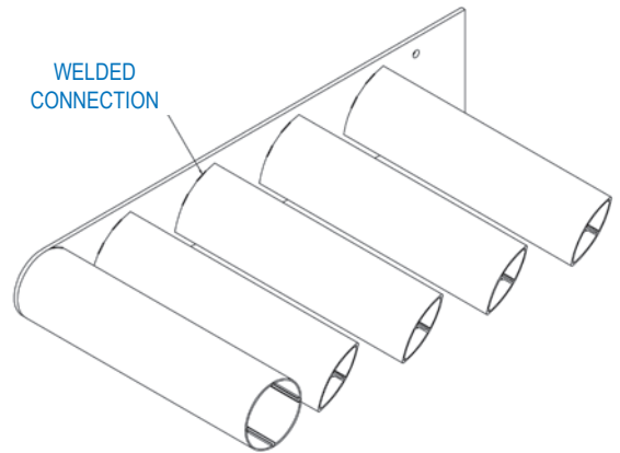
▲ Welded Attachment
